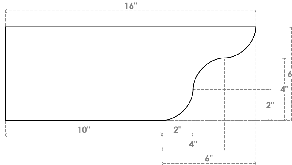
SIDE PROFILE
