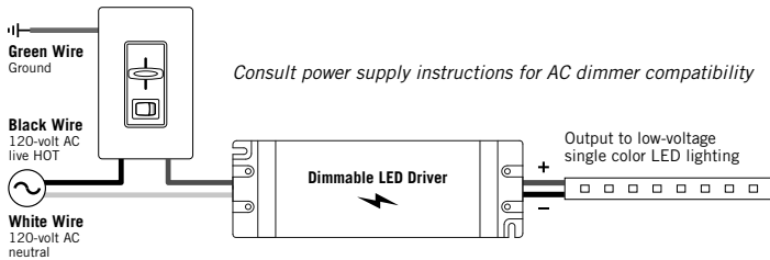
Typical wiring diagram when used with an AC dimmer
