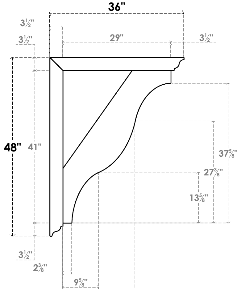
SIDE PROFILE
