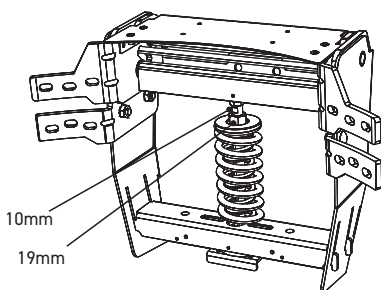
CHARNIÈRE ALTERNATIVE
