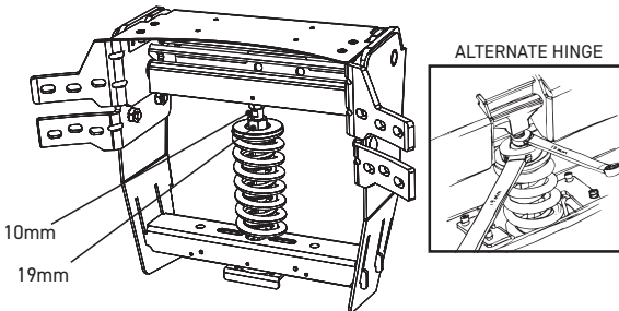
ALTERNATE HINGE
