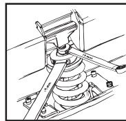
ALTERNATE HINGE
