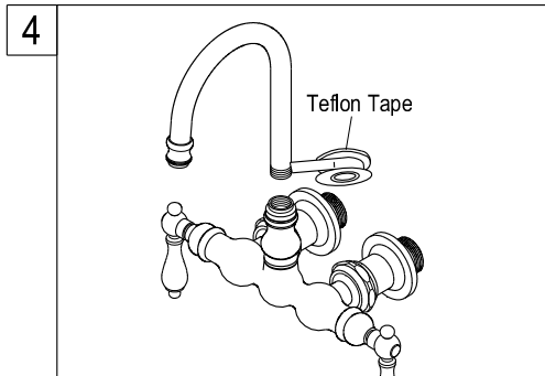
4. Apply Teflon tape to the spout threads then install the spout on top of faucet body.
