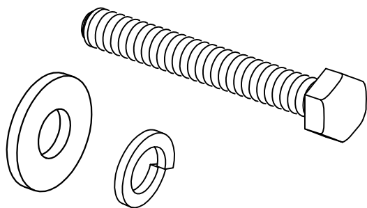
BOLT: M8 X 60mm - QTY 8 LOCK WASHER: Ø12 / Ø8 X 1.5mm - QTY 8 WASHER: Ø19 / Ø8 X 1mm - QTY 8 QTY 8 SETS
