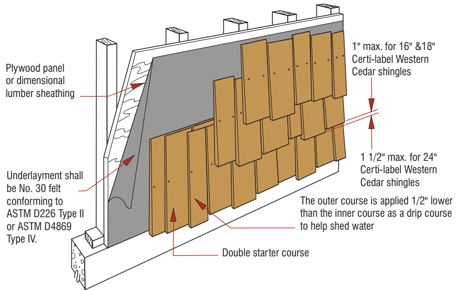
Figure 10: Staggered Coursing
