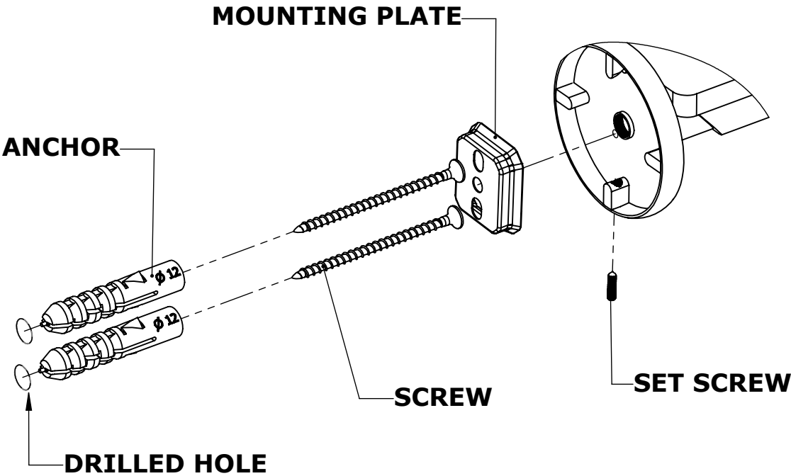
DETAIL M
