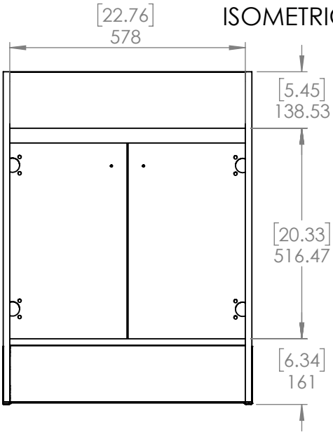
BACK VIEW
