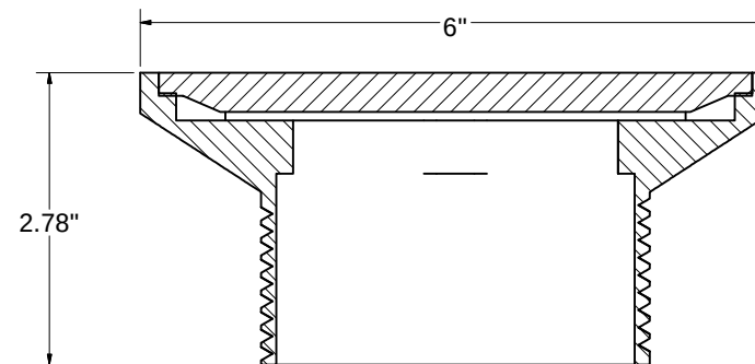
SECTION A-A SCALE 1
