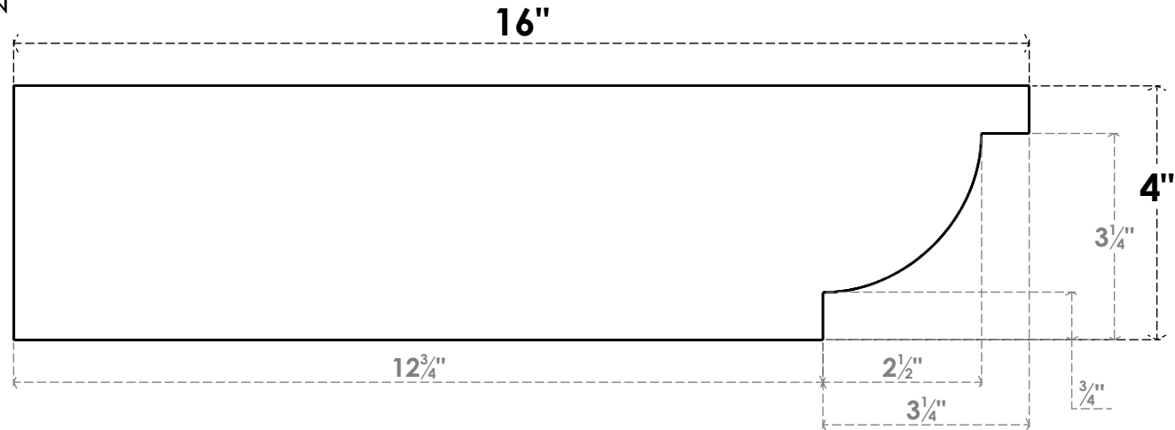
SIDE PROFILE
