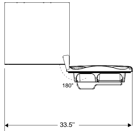
TOP OF REFRIGERATOR WITH DOOR OPEN 180°
