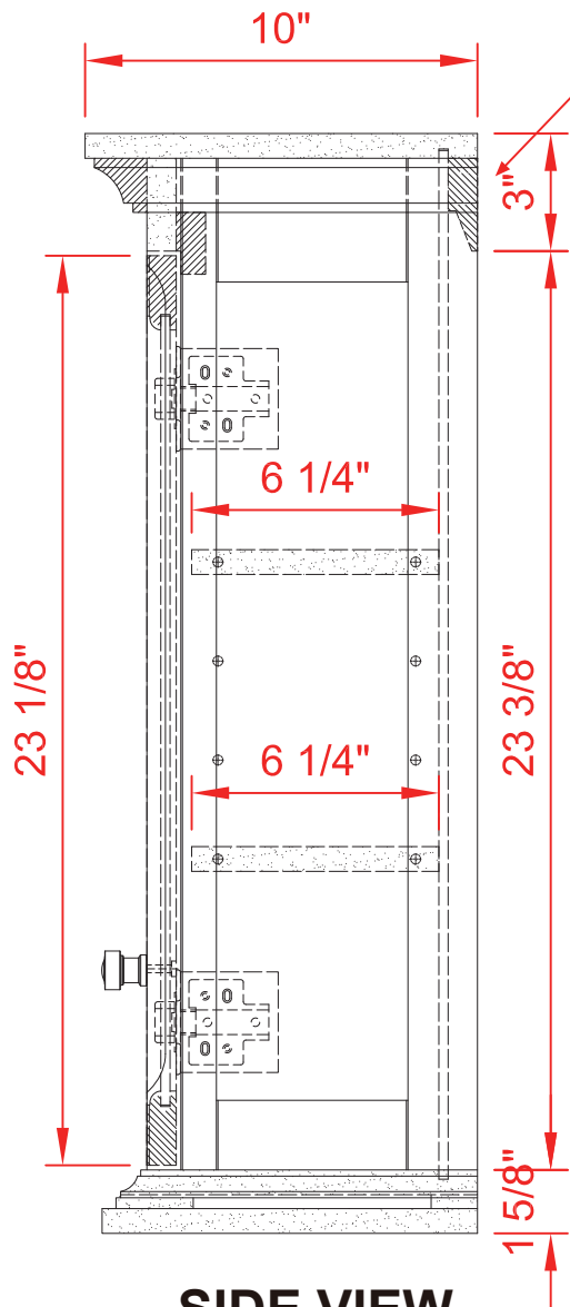
SIDE VIEW
