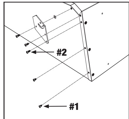
SECURE SIDE PANELS
