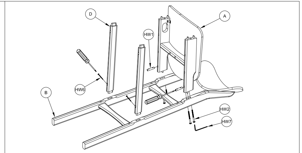
STEP 2: Assemble the seat to the back leg part. Make sure to apply all the bolt into the holes properly before tightening.
