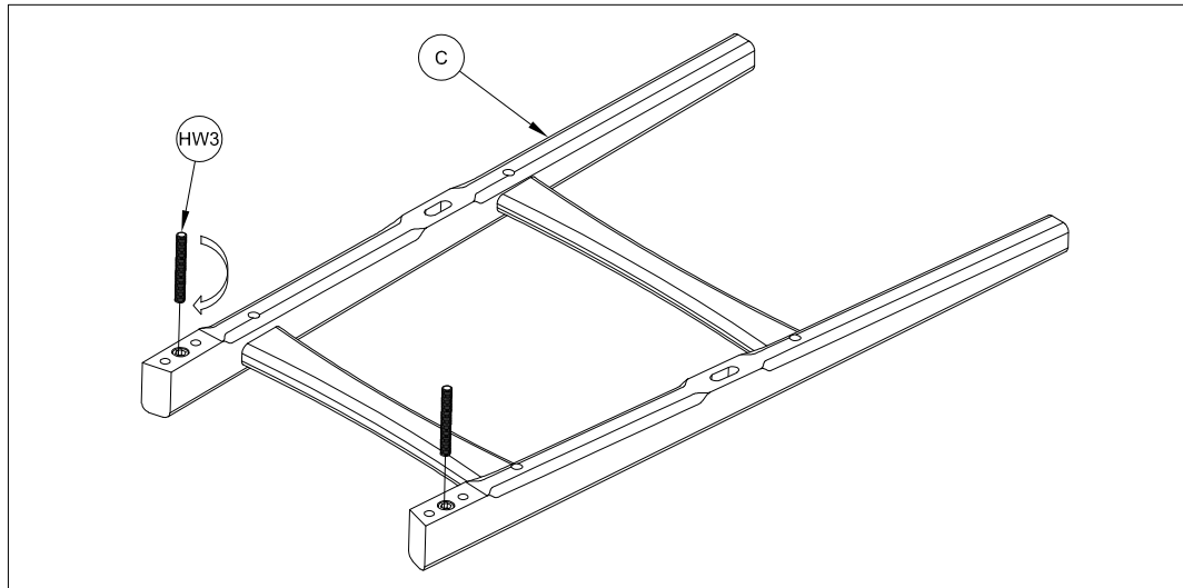
STEP 1: Attach the headless bolts to the front leg part.
