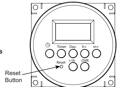
Figure 4. Reset Button
