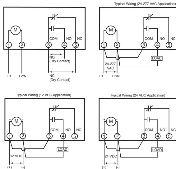
Figure 3. Connect FM1D14 Wiring (Front View Shown).
