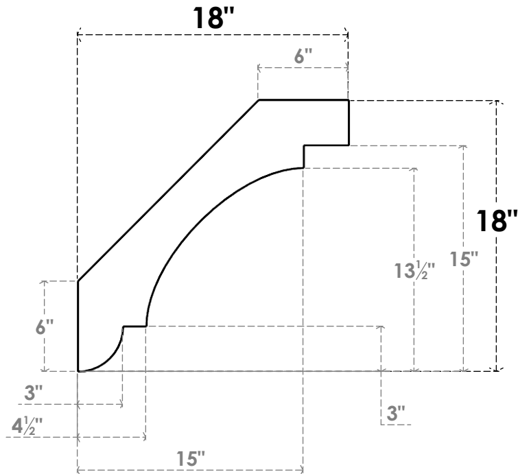
SIDE PROFILE
