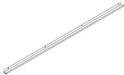
G03 GUTTER - A4M02857 (x1) 1 9/16"x1 15/16"x65 15/16" (40x50x1675)
