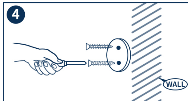
4.TIGHTEN THE STAINLESS STEEL SCREWS WITH A SCREWDRIVER AND FIX THE GASKET
