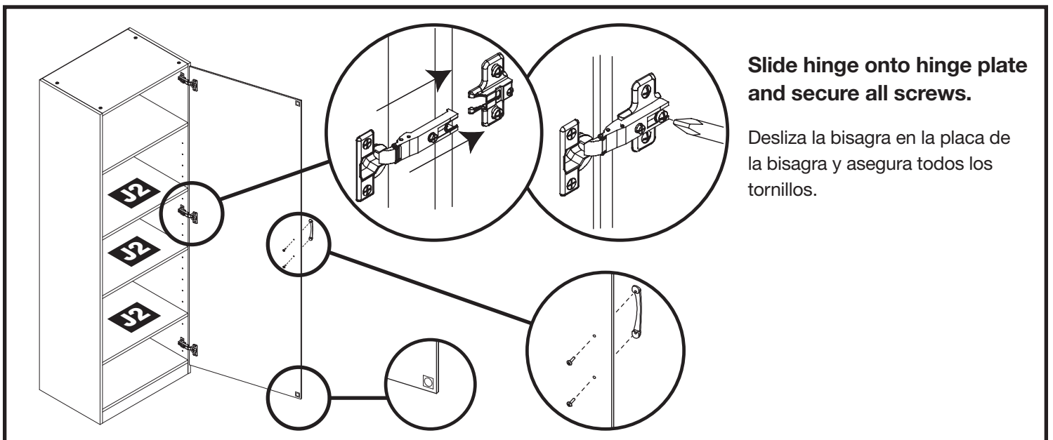
(2) SCREWS (#8-32 x 3/4") TORNILLO
