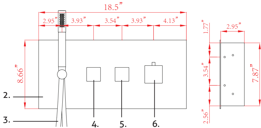
Control Panel
