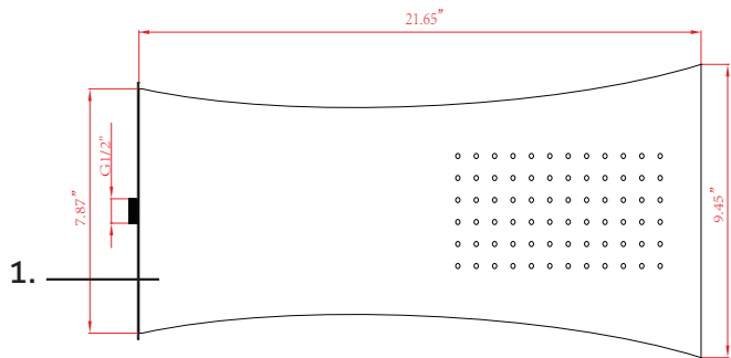
Head Shower
