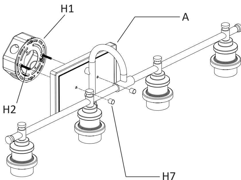
OPTION 1: Mount with glass shades facing down.
