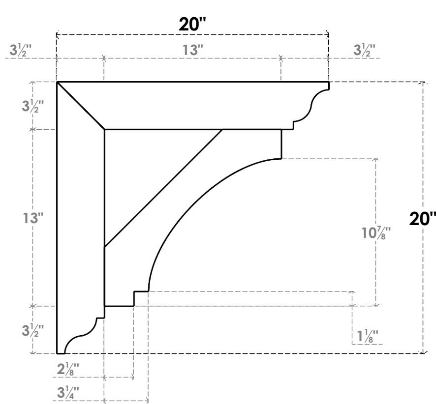
SIDE PROFILE
