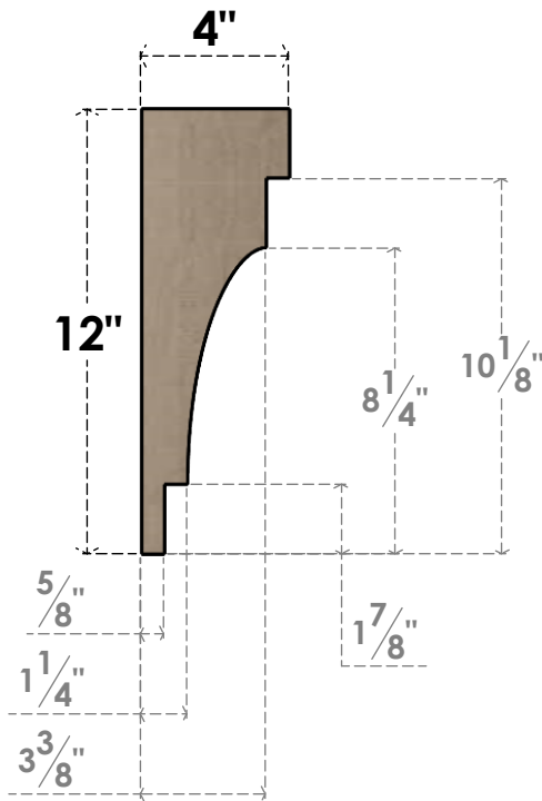
SIDE PROFILE
