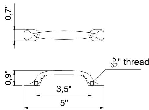
HANDLE
