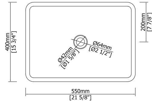
SINK VIEW
