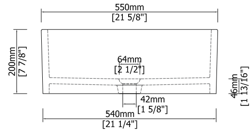
SINK FRONT VIEW
