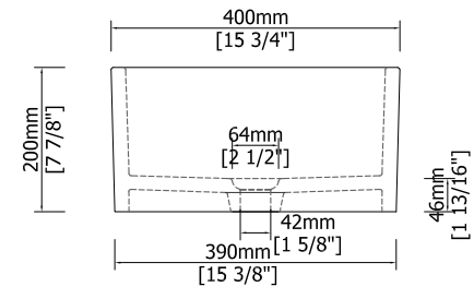
SINK RIGHT VIEW
