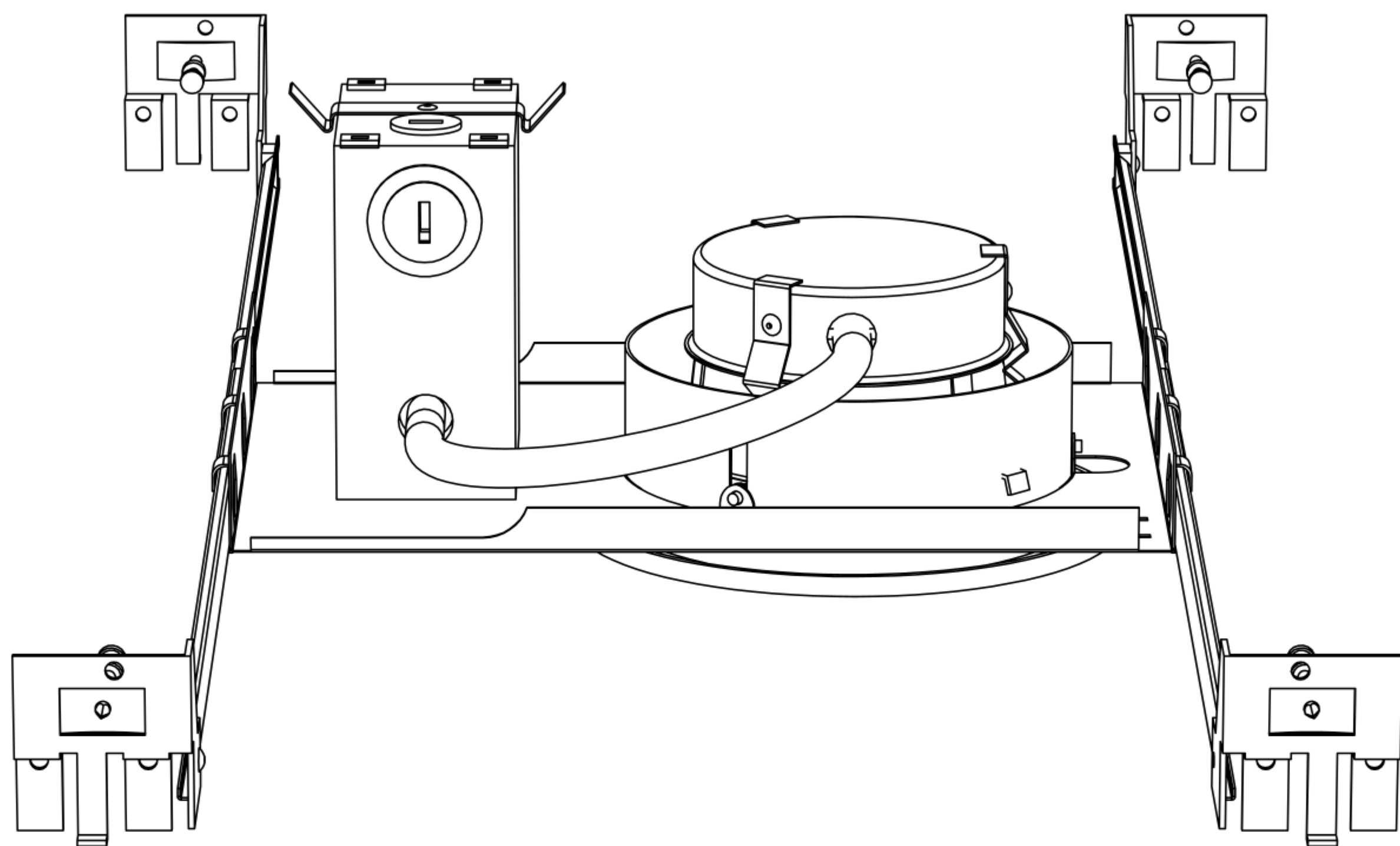
View of properly installed downlight system
