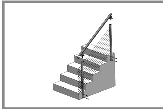
Fascia Mount Stairs 6' Or Less
