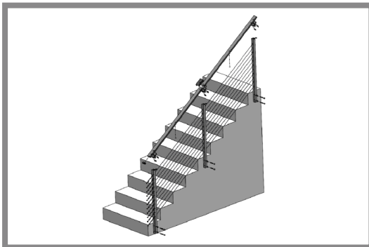
Fascia Mount Stairs 6'- 12'
