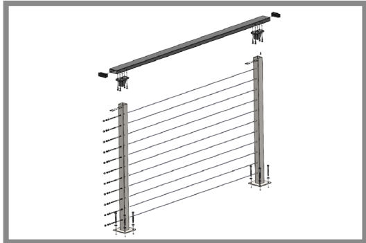
Base Mount Horizontal 6' Or Less
