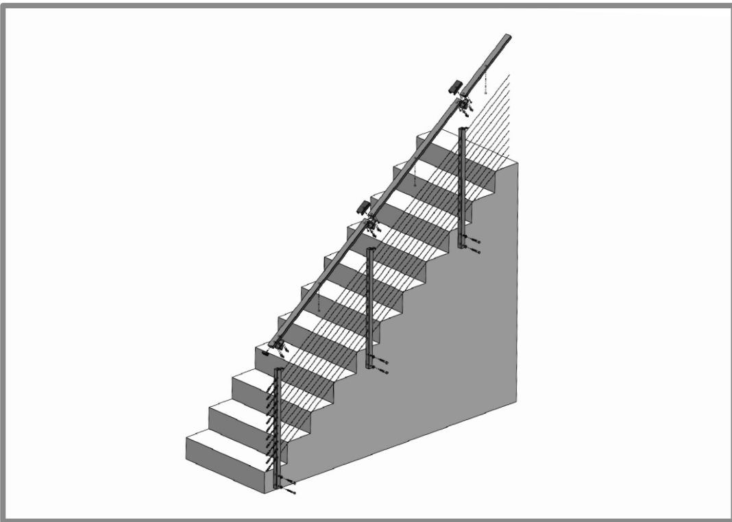
Fascia Mount Stairs Over 12'
