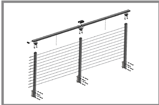
Fascia Mount Horizontal 6'- 12'
