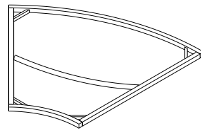
Seat frame (8 pcs)
