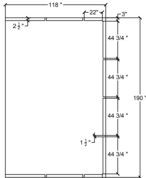
PLAN A LA BASE PLAN AT THE BASE
