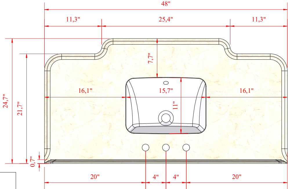
Top View
