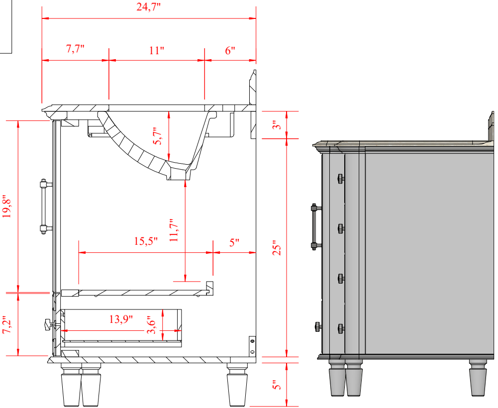
Side View
