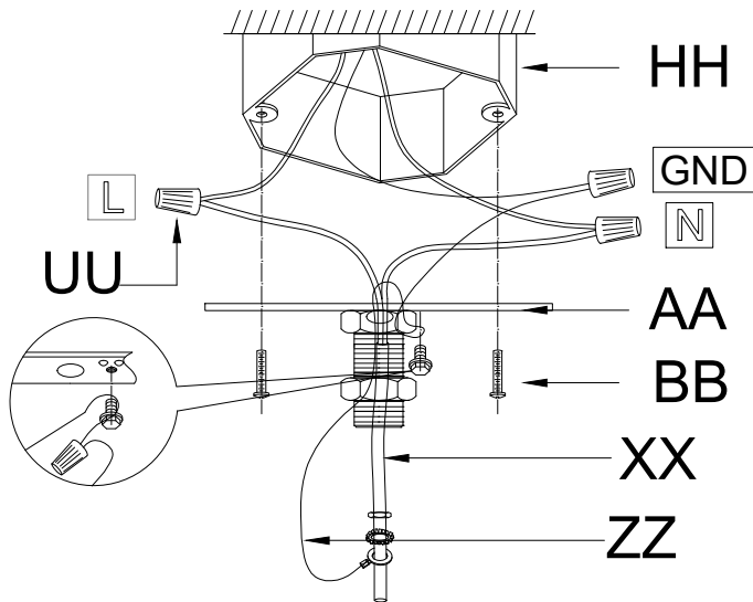
Wire Connection Diagram:
