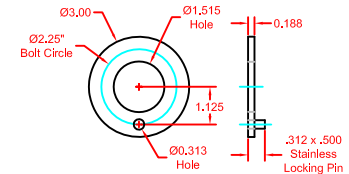
GSSA-Swing Arm Flange with 5/16" Locking Pin
