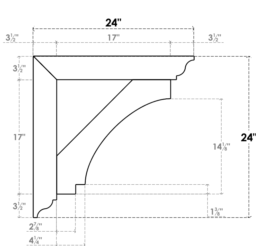
SIDE PROFILE
