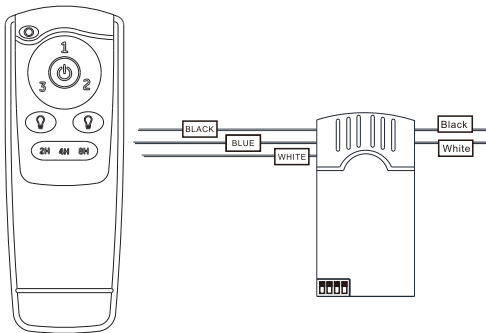
REMOTE CONTROL(1PCS)
