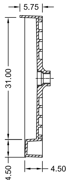
SECTION B-B
