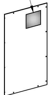
RIGHT BACK PANEL QTY 1
