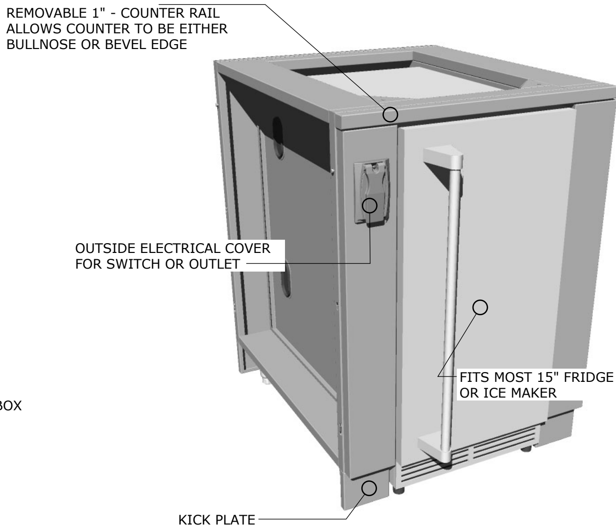
FRONT VIEW
