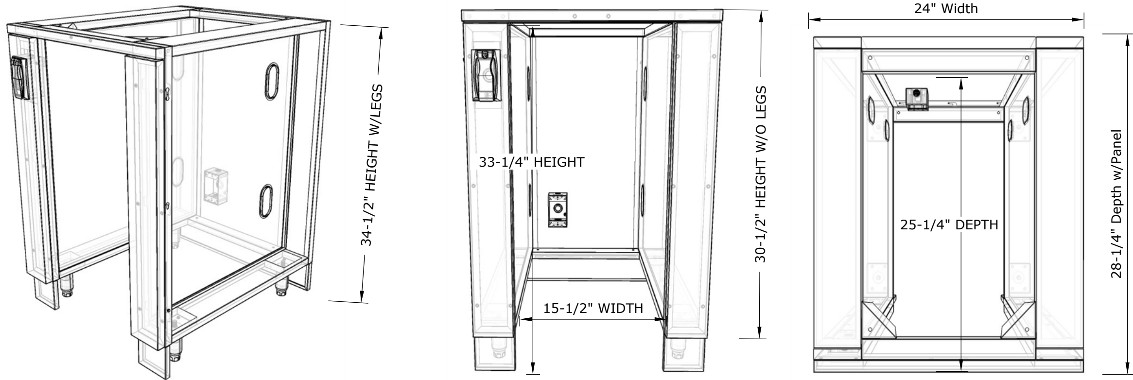
ISO VIEW
