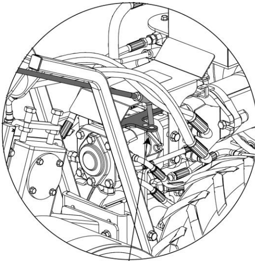
Install Wheel Control Rod Into Bracket on right side
