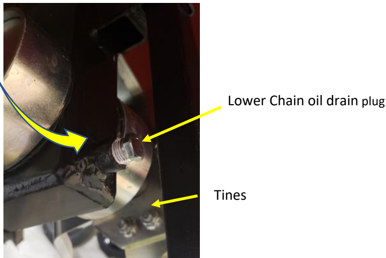
Under side of Tiller Tine/Shroud
