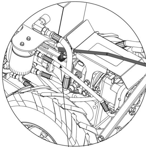
Install Tine Control Rod Into Bracket on left side
