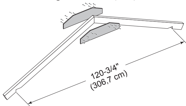
Fig. B - Build 11 (total)
