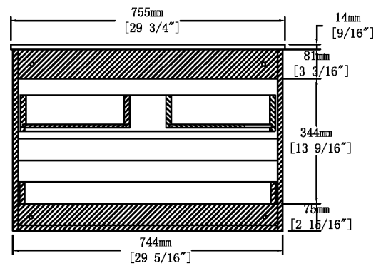
Back View
