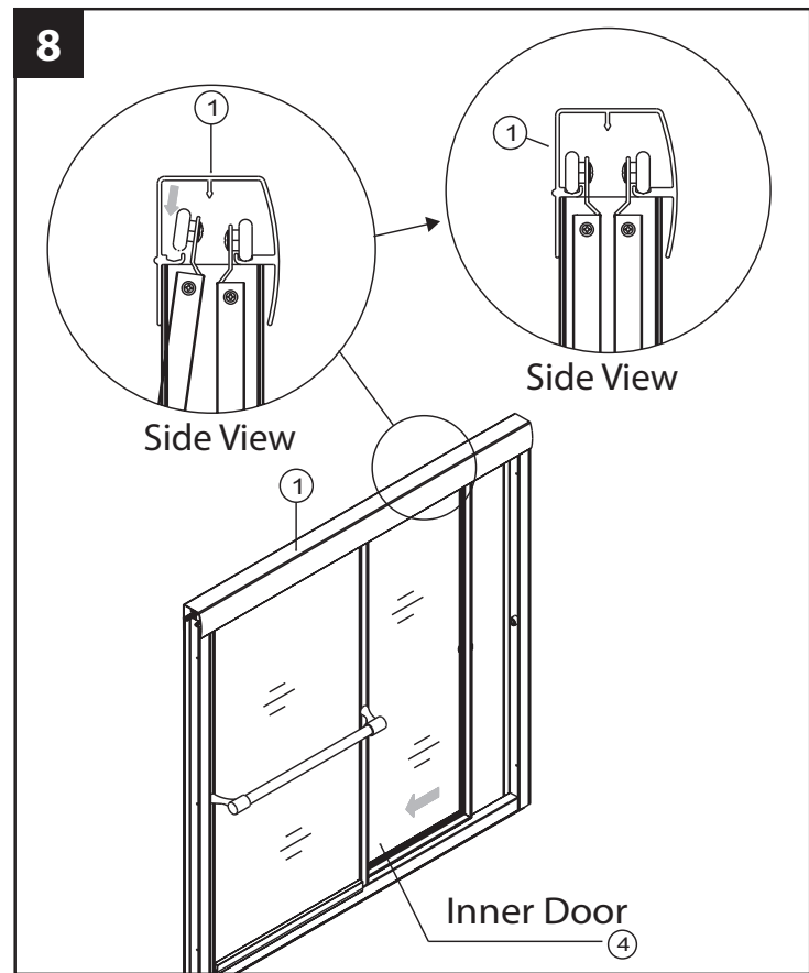
8. Install inner door panel by lifting up and into top track as shown.
