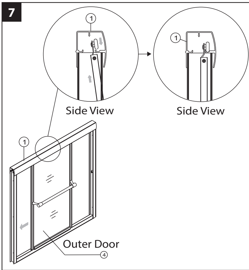
7. Install outer door panel by lifting up and into top track as shown.
