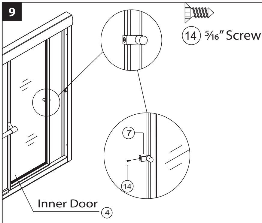
9. Attach knob to the end of the inside panel that is opposite of shower head.
