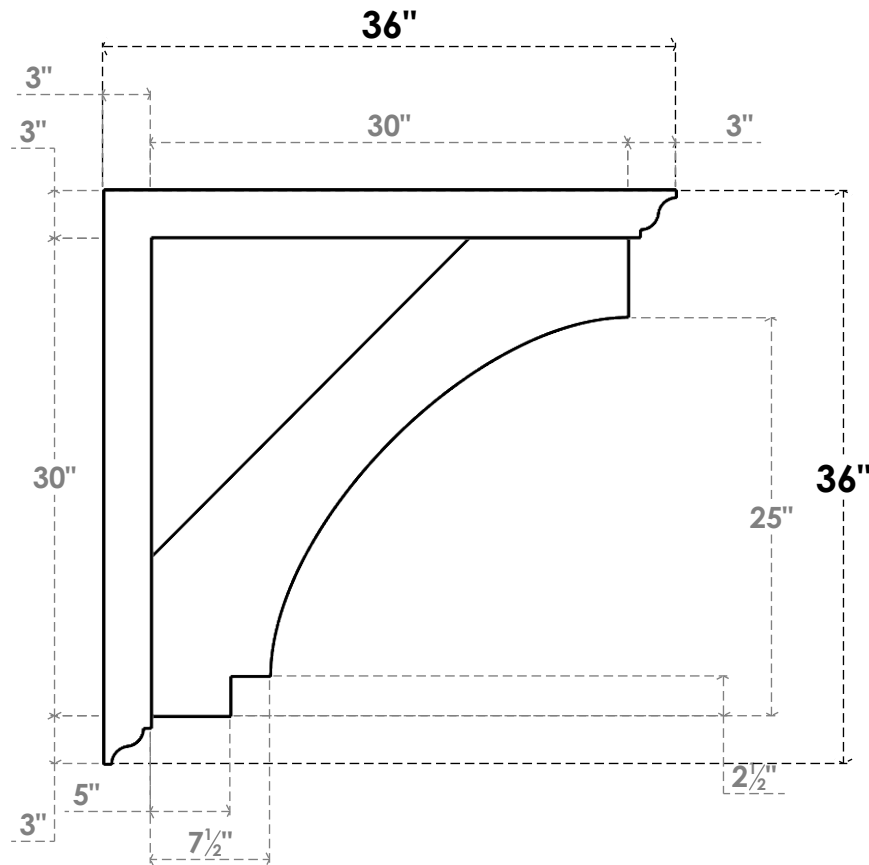
SIDE PROFILE
