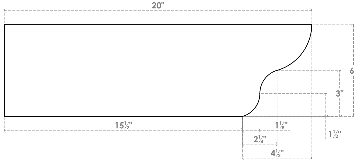
SIDE PROFILE
