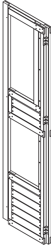
1pc. - 9264 - 63.5 x 558.8 x 2286mm 2-1/2 x 22 x 90" Folding Panel Assembly Left A - 37569264
