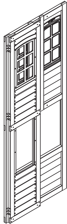
1pc. - 9265 - 63.5 x 866.6 x 2286mm 2-1/2 x 34-1/4 x 90" Folding Panel Assembly Left B - 37569265
