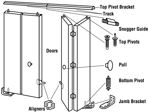
Double bifold units can be mounted together for openings up to 72" wide
