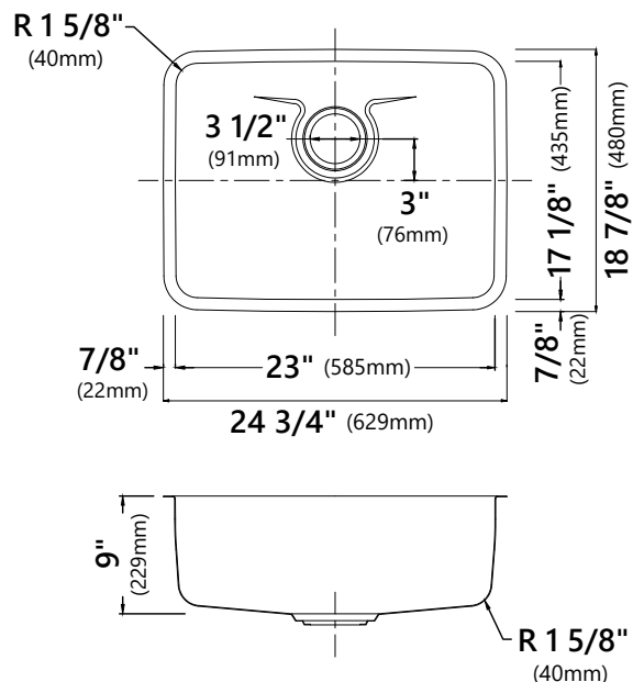
KD1US25B 24 3/4" x 18 7/8" x 9" Min Cabinet Size: 30"
