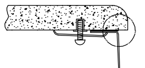
1/8" Negative Reveal
