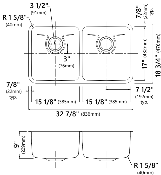
KD1UD33B 32 7/8" x 18 3/4" x 9" Min Cabinet Size: 36"
