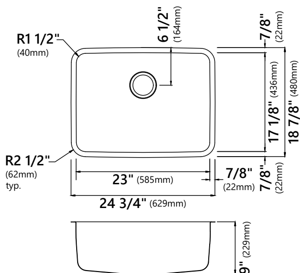
KA1US25B 24 3/4" \times 18 7/8" \times 9" Min Cabinet Size: 30"
