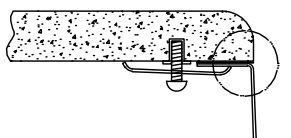
Flushed/Zero Reveal
