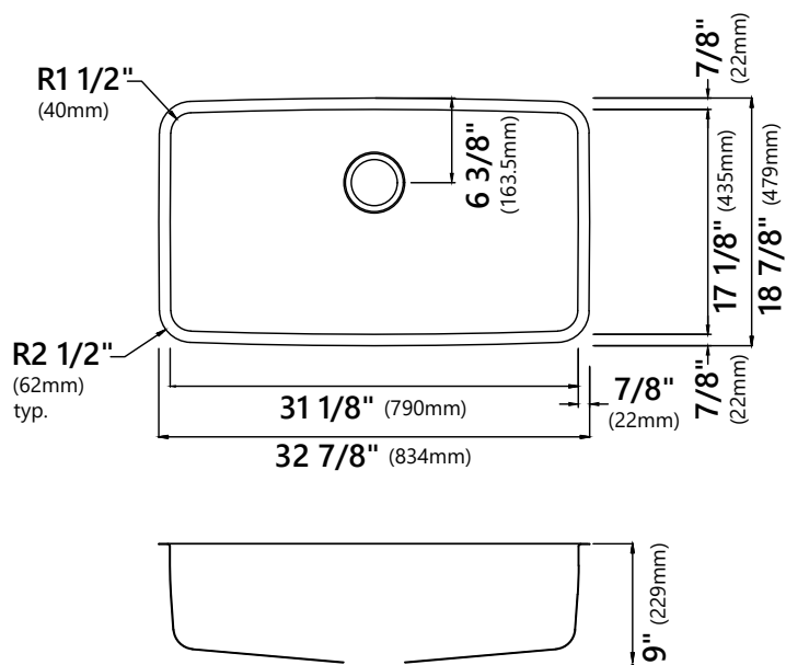
KA1US33B 32 7/8" \times 18 7/8" \times 9" Min Cabinet Size: 36"
