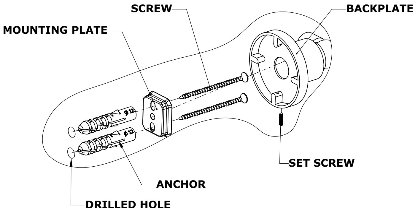
DETAIL O
