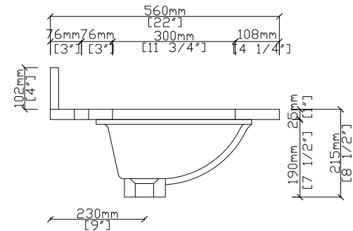
RIGHT VIEW
