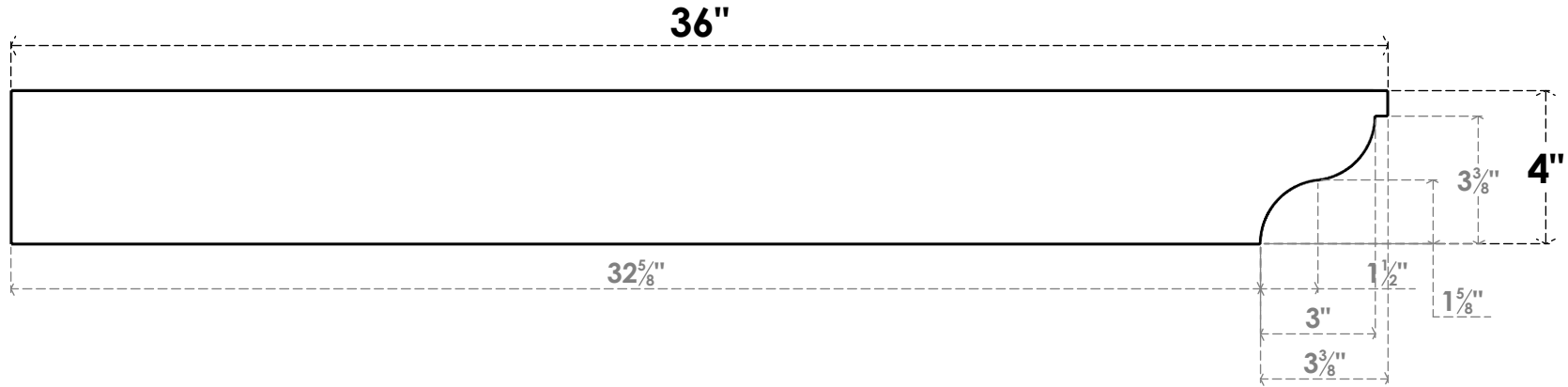
SIDE PROFILE
